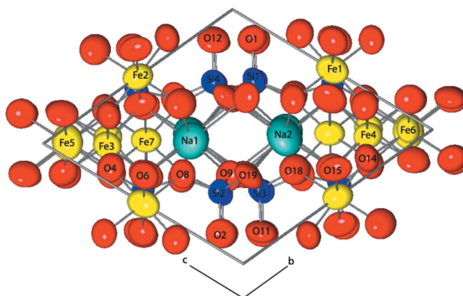
Figure 1 The crystal structure of wilkinsonite, viewed down the [100] direction. Displacement ellipsoids are drawn at the 99.9999% probability level.
